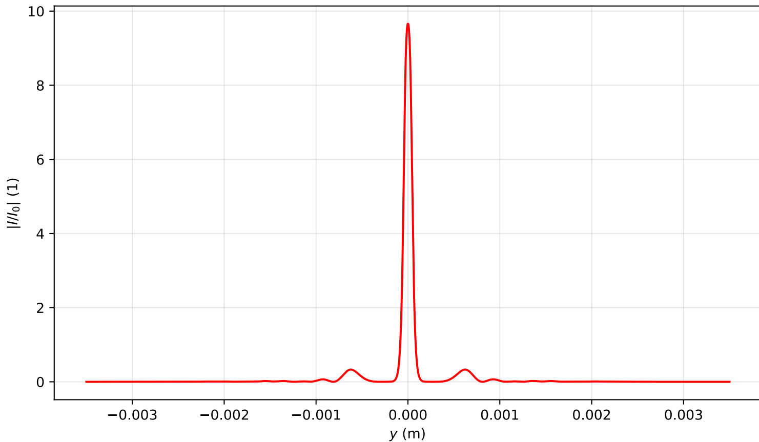
Intensity profile I(x=0, y, z=0.478)/I_0 , P_{in}=7.0P_{cr} , artificial time
